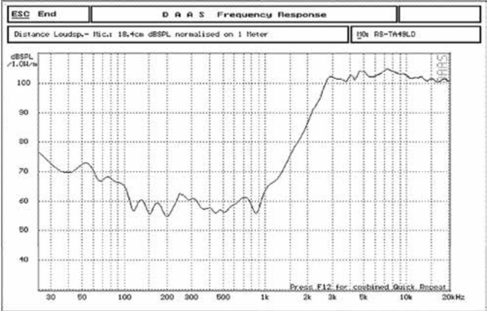
SPL vs. FREQ
